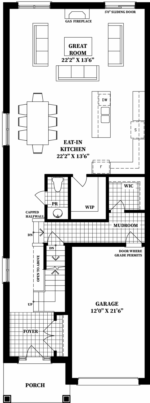
Ground Floor
